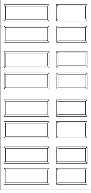
14'0" x 7'0" (4276 x 2134)
