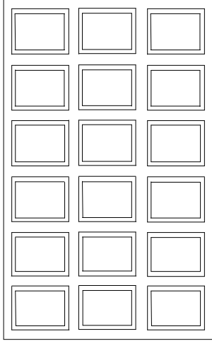
110" x 70" (3353 x 2134)
